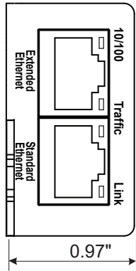
Left View
