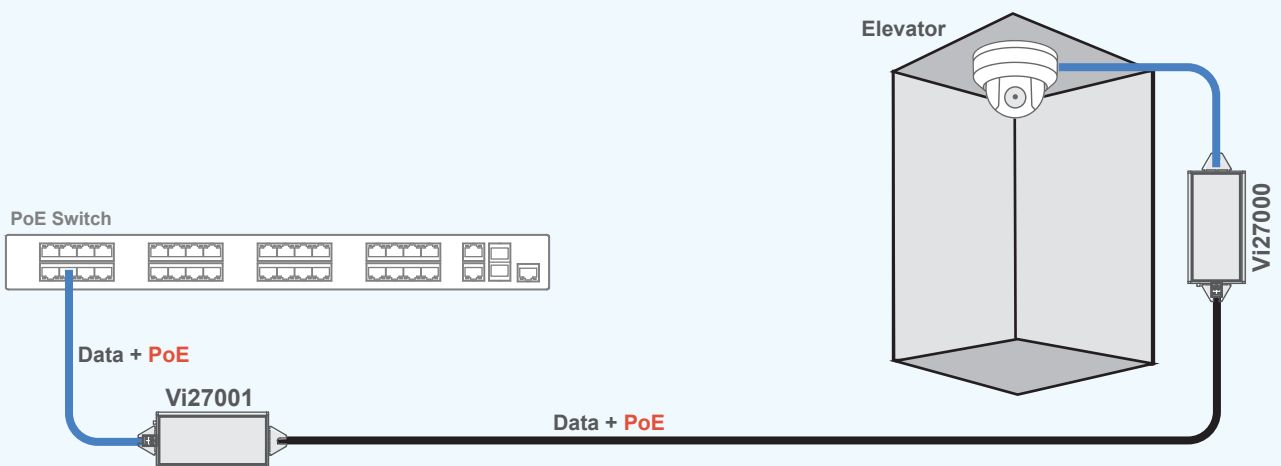
The Vi27000 series can transmit Ethernet and PoE over a wide variety of single pair wires.
