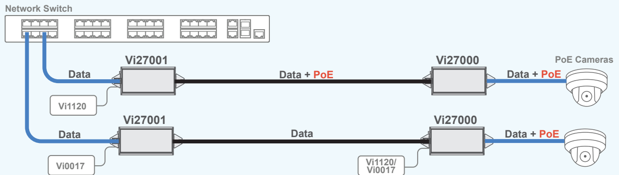
Both the Vi27001 and the Vi27000 can use local power supplies to power themselves and provide PoE to the IP camera. The Vi27001 receiver can use a local power supply to power Vi27000 transmitter and the IP camera using PoE.
