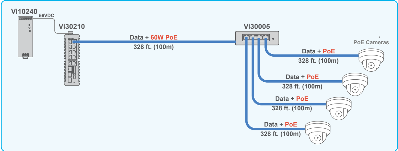
The Vi10240 can be used to power a local PoE switch, a remote PoE powered PoE switch and multiple connected PoE cameras.
