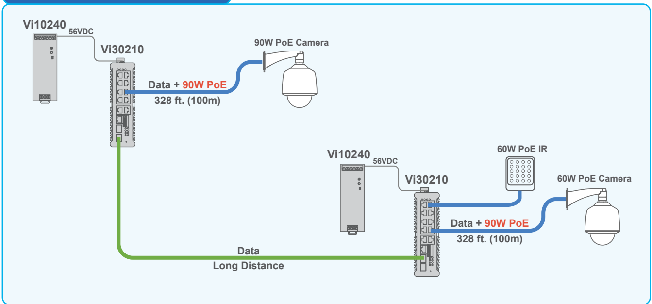
Multiple Vi10240s can be used in a wide variety to power High power cameras and IR illuminators.
