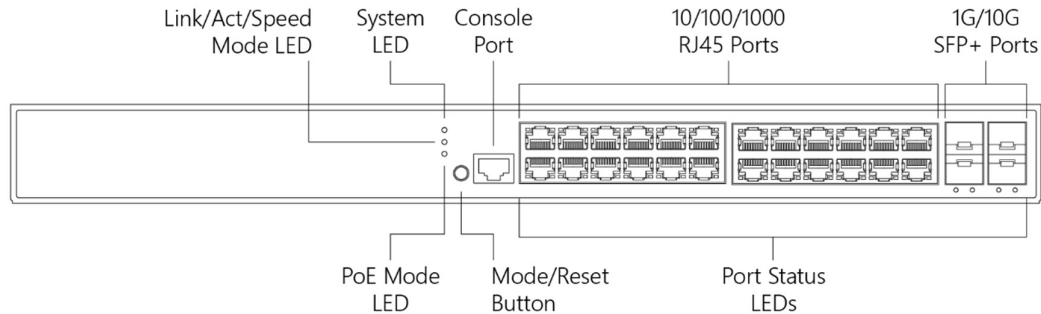
Figure 1: Front panel of the switch
