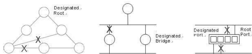
Figure 7: The Spanning Tree Protocol
