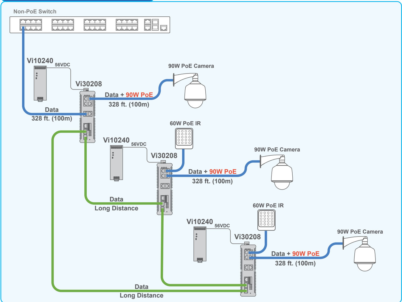
Multiple Vi30208s can be used in a Ring Network configuration to increase their reliability of the network.
