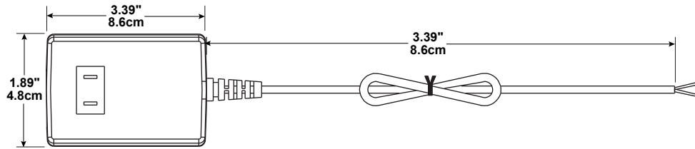
Rear View
