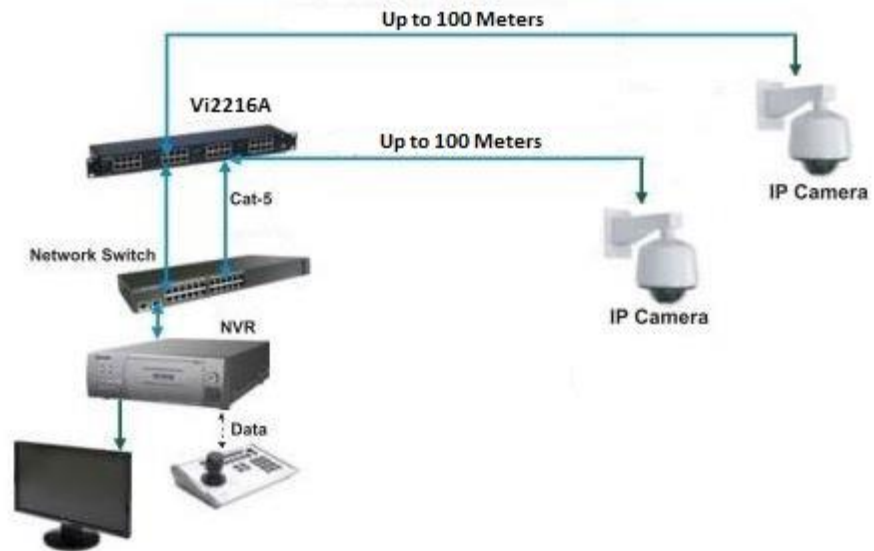
Figure 5: Vi2216 Application Drawing
