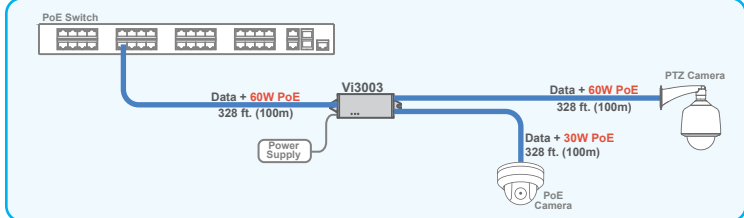
Vi3003 allows for the transmission of two cameras over a single cable run or adding a new
