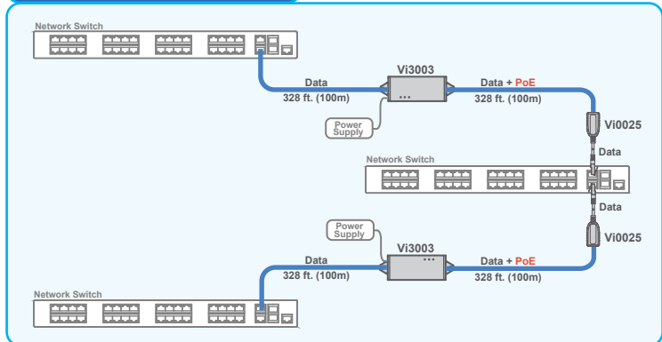
Vi3003 enables extending 1G connection between networks.
