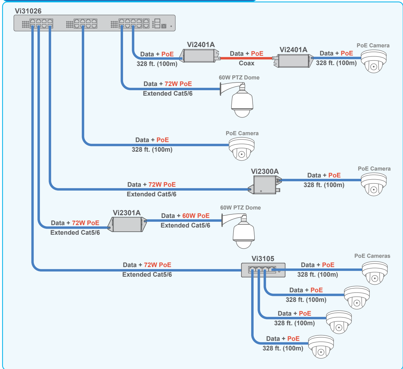
The Vi32026 can transmit data and PoE up to 72W over standard and extended UTP cables.
