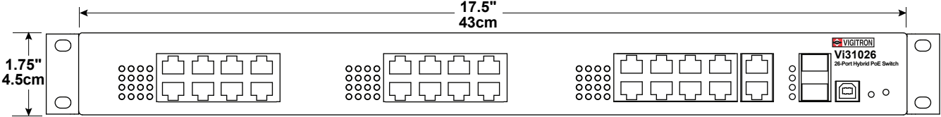
Front View
