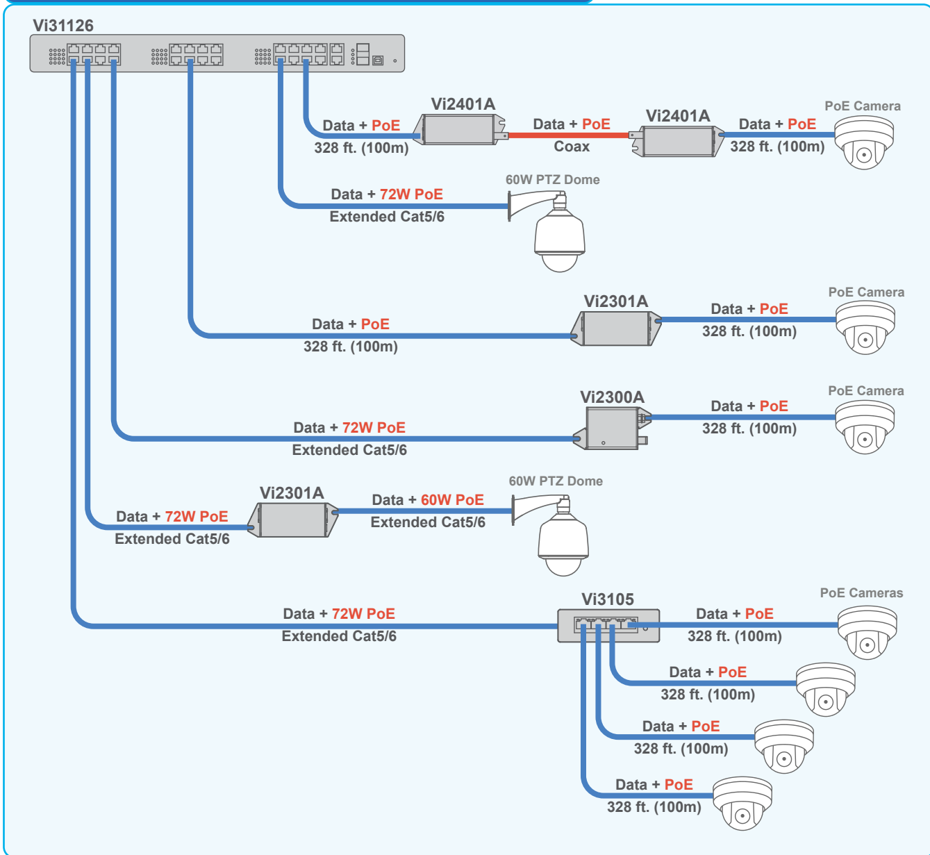
The Vi31126 can transmit data and PoE up to 72W over standard and extended UTP cables.
