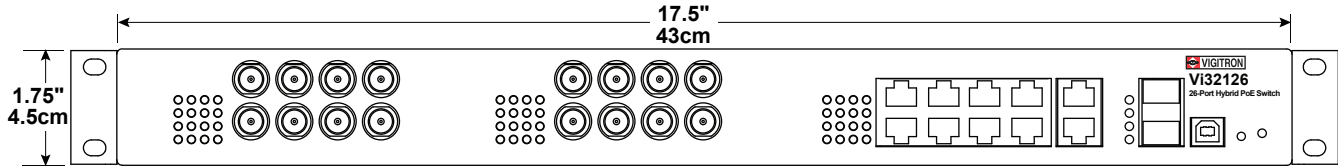
Front View
