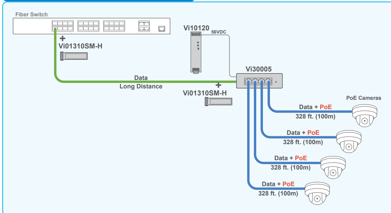
The Vi01310SM-H can provide long distance connection over fiber cables.
