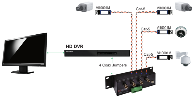
Vi10004: 4-Ch. Passive HD Transceiver Hub
