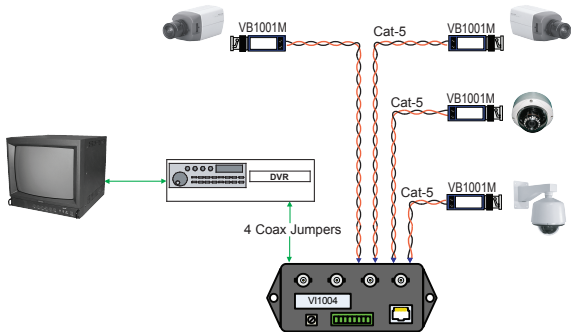
Vi1004: 4-Ch. Passive Receiver
