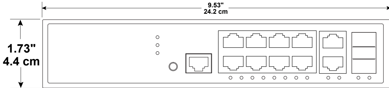
Front View
