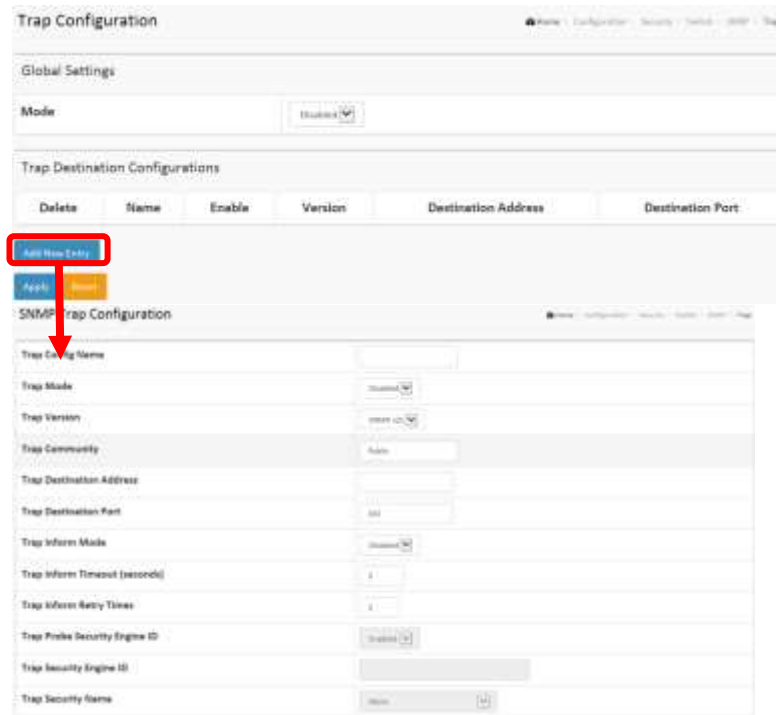
Figure 2.5.1.5.2: The SNMP Trap Configuration
