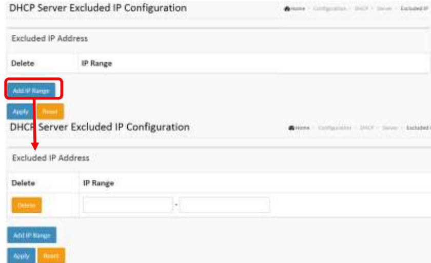
Figure 2.4.1.2: The DHCP Server Excluded IP
