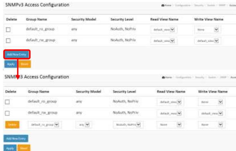
Figure 2.5.1.5.7: The SNMP Accesses Configuration
