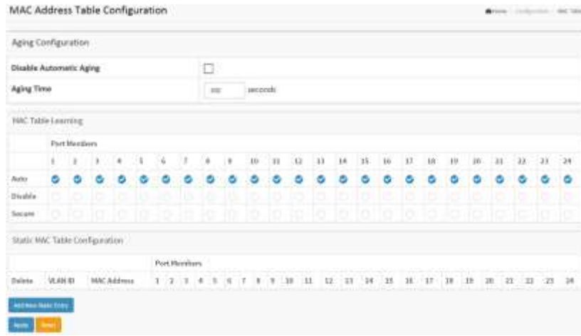
Figure 2.14: The MAC Address Table Configuration
