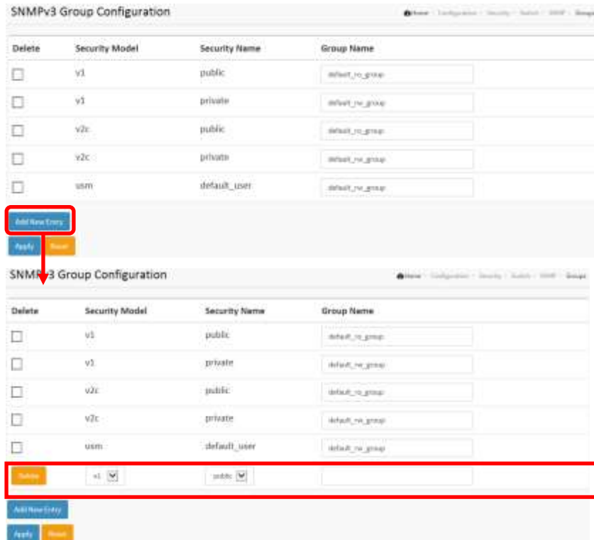
Figure 2.5.1.5.5: The SNMP Groups Configuration
