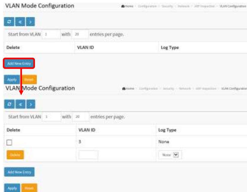
Figure 2.5.2.5.2: The VLAN Mode Configuration
