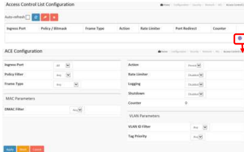
Figure 2.5.2.3.3: The ACL Rate Limiter Configuration
