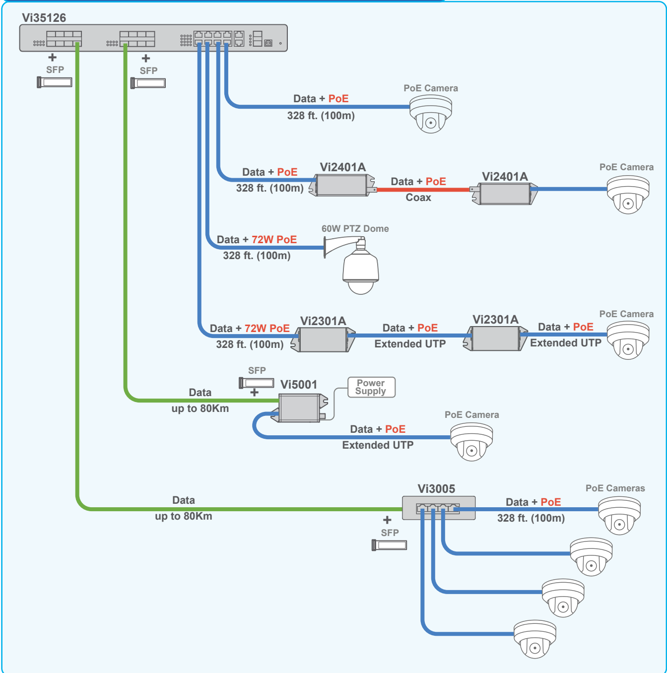
Vigtron media converters and switches with Fiber connection can be used with Vi35126 to provide PoE to cameras or other PoE devices.
