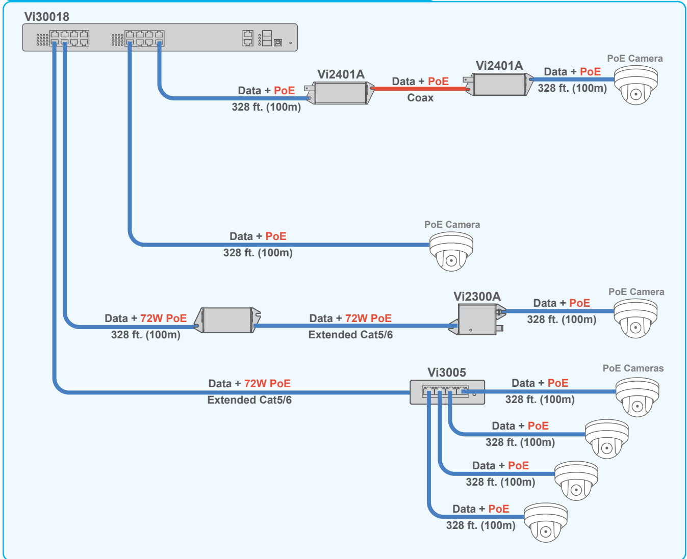
The Vi30018 can transmit data and PoE up to 72W over standard UTP cables.
