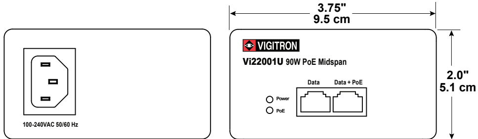
Left View
