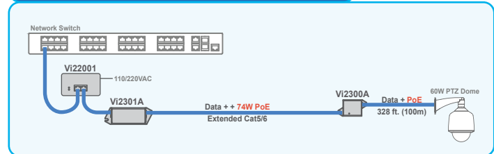
The Vi2300A extends Ethernet and 74W PoE from a PoE Midspan.
