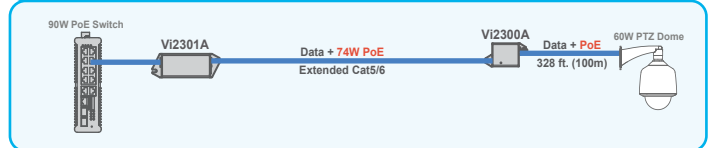
The Vi2300A extends Ethernet and 74W PoE from a PoE switch.
