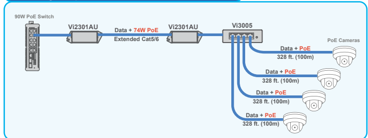
The Vi2301As and Vi3005 can be used to connect multiple PoE cameras at extended distances.
