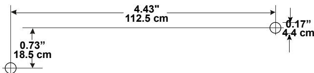
Mounting Pattern
