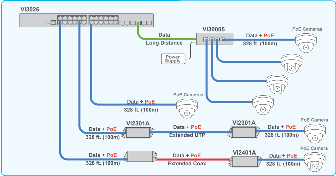
The Vi3026 can provide can be used to connect IP cameras over fiber optics and Extended UTP and Coax.
