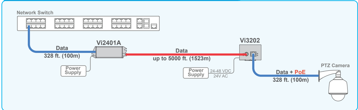
Vi3202 along with Vi2401A can be used to provide data and PoE transmission over long distance coax cables.
