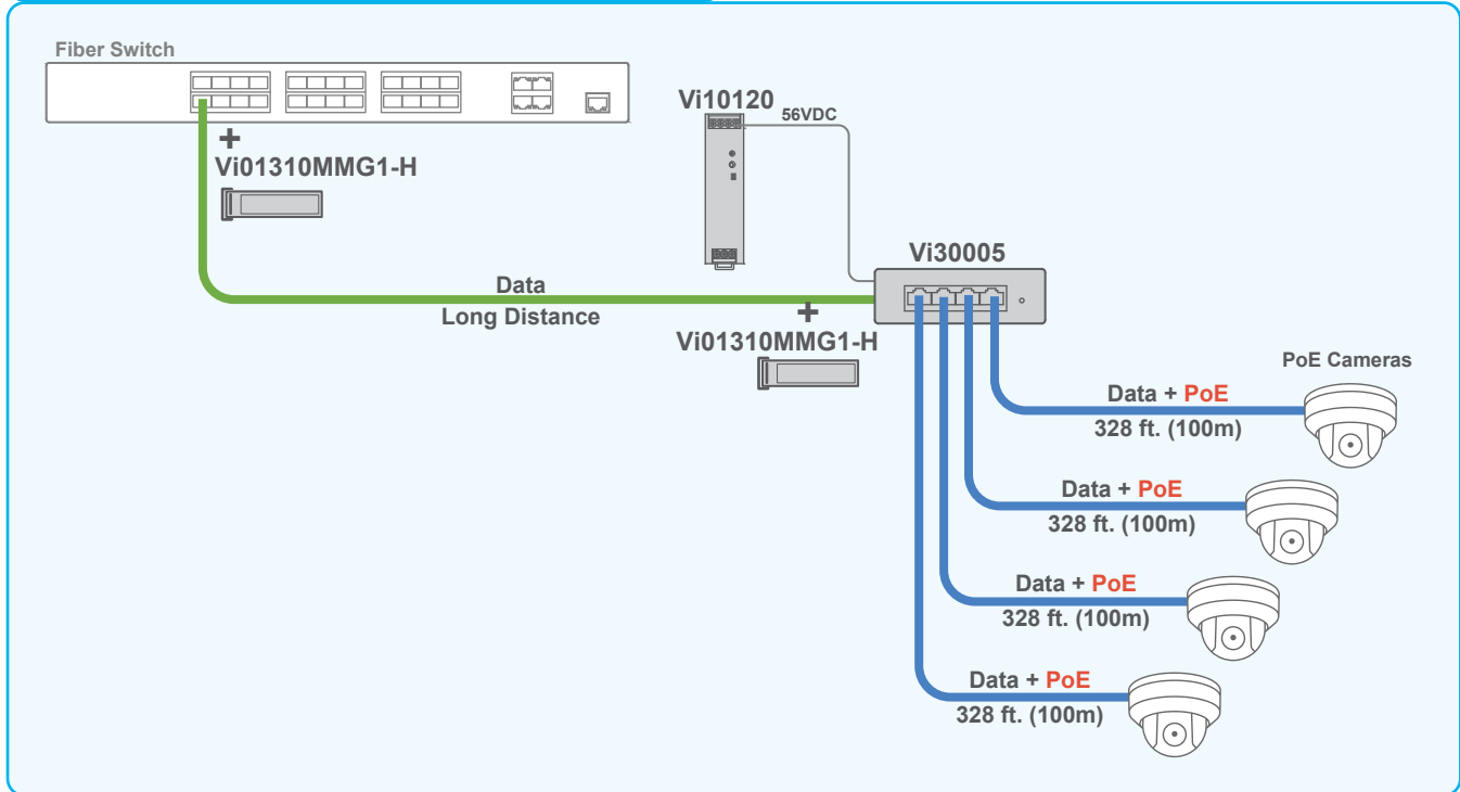
The Vi01310MMA-H can provide long distance connection over fiber cables.
