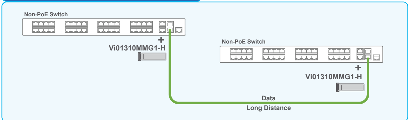
The Vi01310MMA-H can connect 2 network switches at long distances at 1000Mbps data rate.
