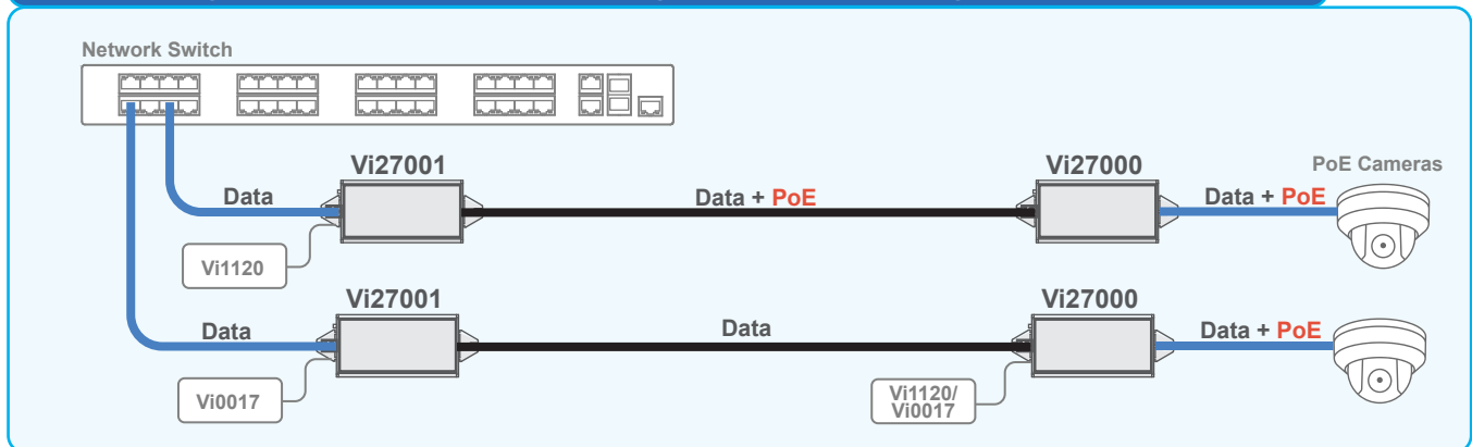
Both the Vi27001 and the Vi27000 can use local power supplies to power themselves and provide PoE to the IP camera. The Vi27001 receiver can use a local power supply to power Vi27000 transmitter and the IP camera using PoE.
