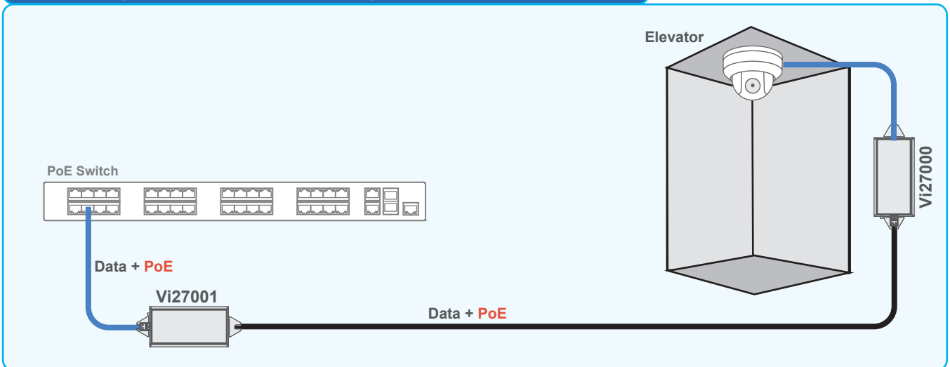
The Vi27000 series can transmit Ethernet and PoE over a wide variety of single pair wires.
