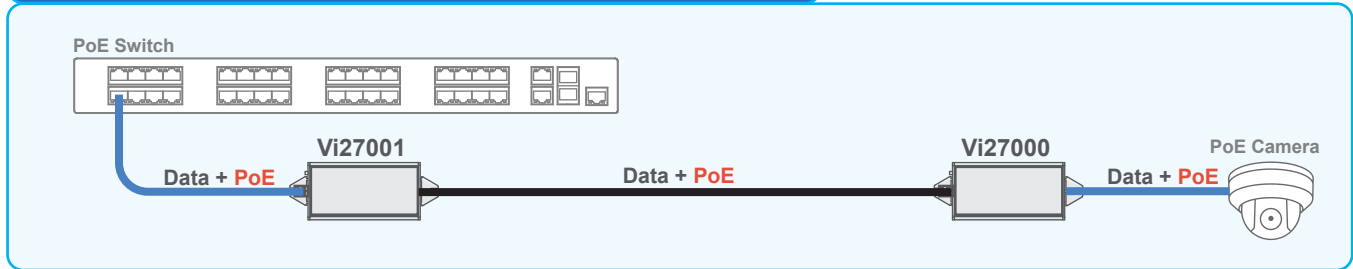
The Vi27000 series and a IP camera can be powered by a PoE switch.
