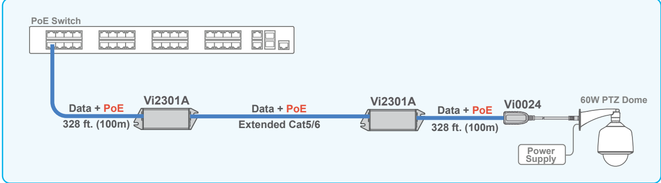
The Vi0024 can be used to power Ethernet Extenders using PoE when the end point is a Non PoE device.
