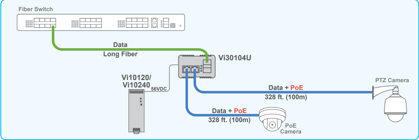
Vi30104U allows for the transmission of two cameras over a single Fiber cable or adding a new camera close to an existing camera.
